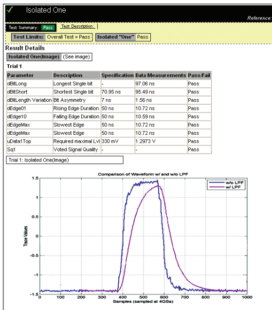
Figure 10: Test report from Keysight's FlexRay Physical Layer Conformance Test software package.
