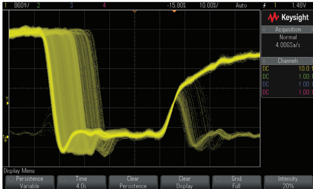
Figure 1: An update rate of 1,000,000 waveforms/sec easily captures infrequent glitches and jitter that other scopes miss.
