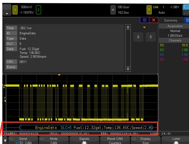
Figure 7: Real-time frame counter and bus utilization measurement helps characterize CAN and FlexRay systems.
