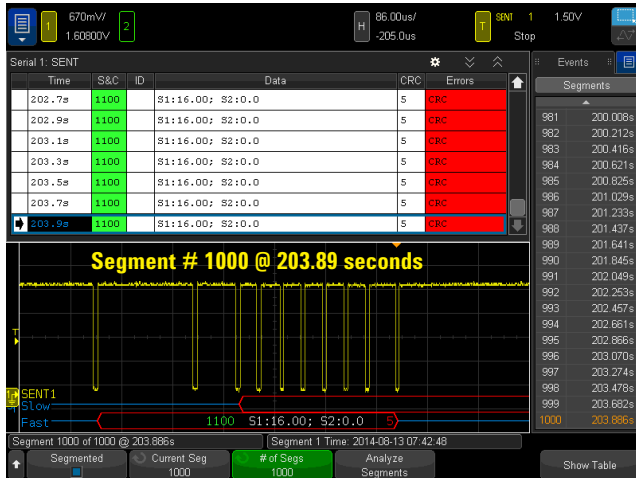
Figure 8: Segmented memory acquisition with automatic decoding selectively captures 1000 consecutive occurrences of SENT fast-channel CRC errors with precise time-tagging between each occurrence.
