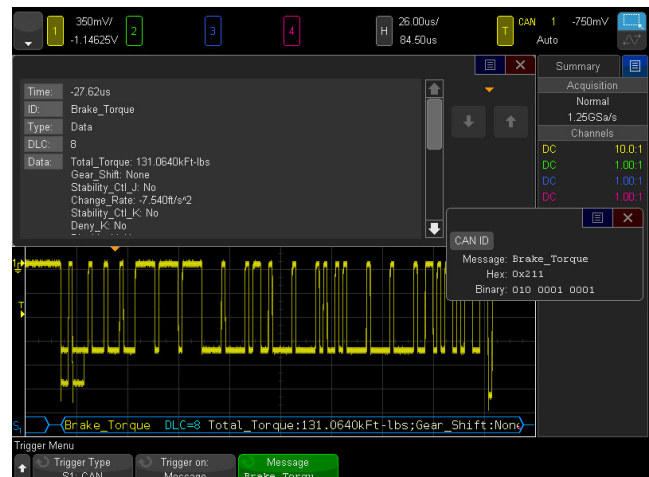
Figure 3: CAN-dbc symbolic decode and trigger.
